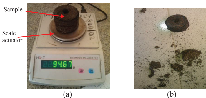
Figure 5 Set-up during shatter index test (a) Weighing of sample before test (b) Shattered sample after the test
