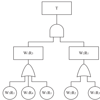
Figure 4 Fault tree
