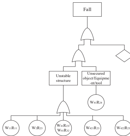
Figure 8 Fault tree of fall
