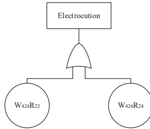
Figure 10 Fault tree of electrocution
