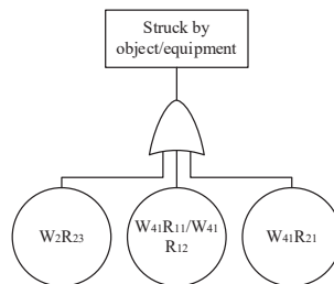
Figure 9 Fault tree of struck by object/equipment
