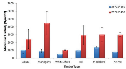
Figure 4: Elastic Modulus Results for Varying Sections of the Timber Species
