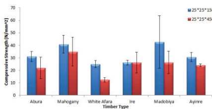
Figure 3: Compressive Strength Results for Varying Sections of the Timber Species
