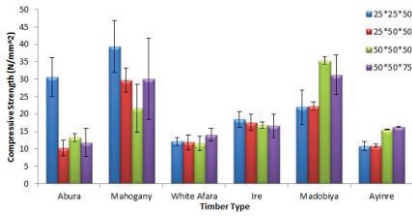
Figure 6: Compressive Strength for Varying Section of the Timber Samples
