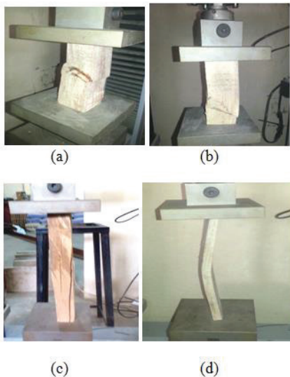
Figure 5: (a) Typical shearing, (b) crushing, (c) splitting and (d) buckling failure modes of timber samples oriented parallel to grain and under compression
