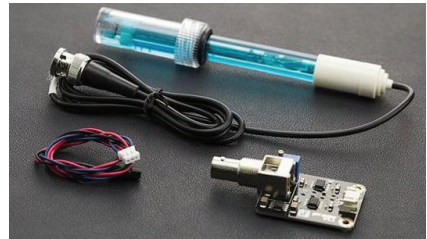
Figure 2: pH sensor
