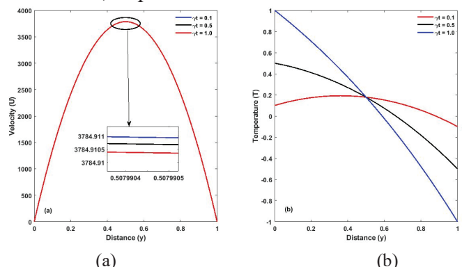
Figure 8: Temperature profiles for \lambda = 100 and different values for \gamma_t
