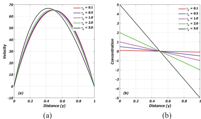
Figure 4: Concentration profile for \xi = 0.01 and S = 2.0 for different values of ( \gamma_c )
