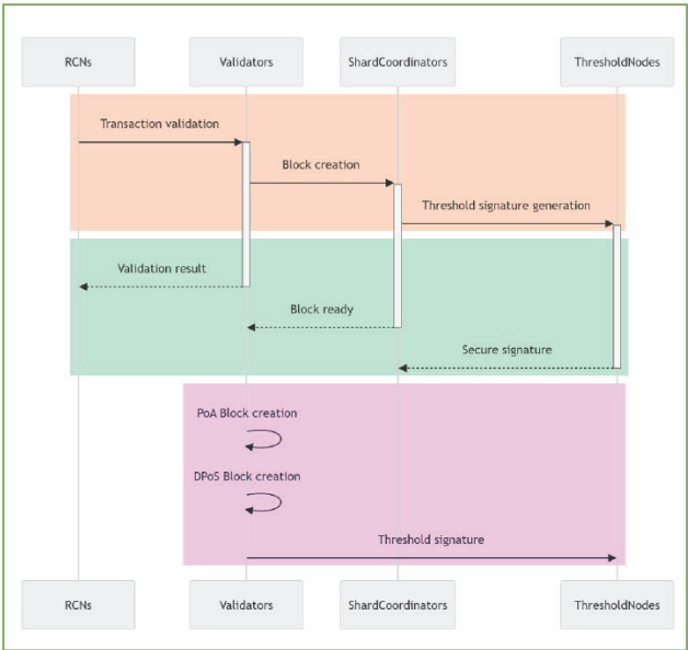
Figure 2: Proposed Architecture Model
