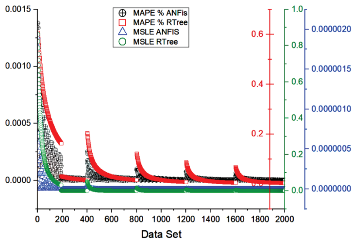
Figure 4: Model Evaluation at the Transportation Stage Using MAPE and MSLE Metrics
