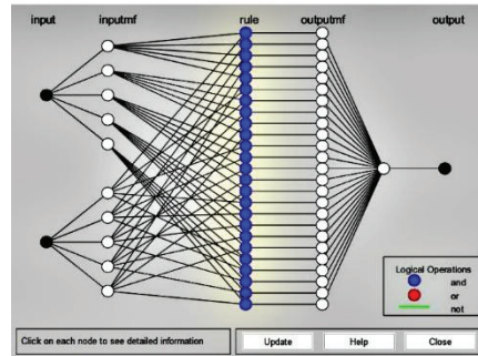
Figure 2: ANFIS Architecture for Carbon Emission Prediction
