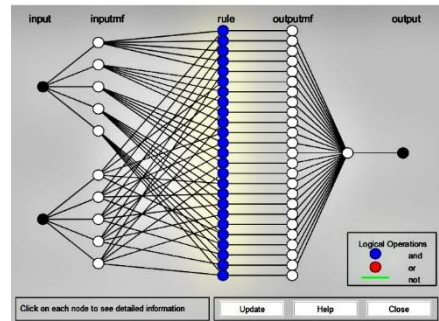
Figure 2: ANFIS Architecture for Carbon Emission Prediction
